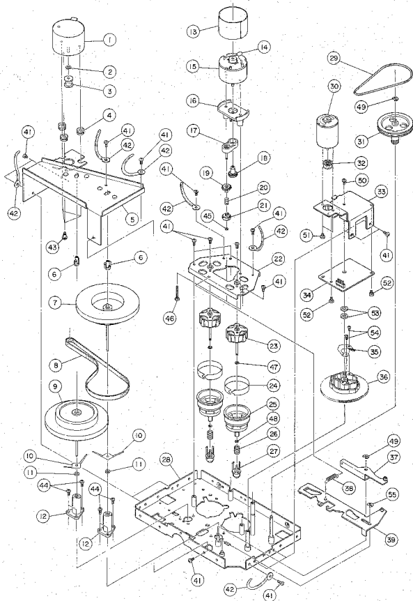
EXPLODED VIEW - 3 (R-9000)
