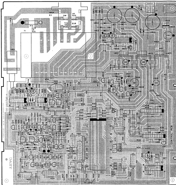
CONTROL PCB
