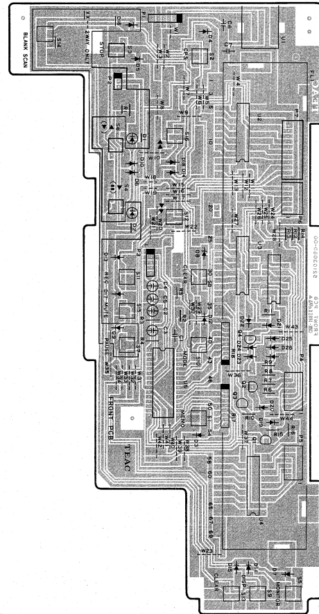
FRONT PCB
